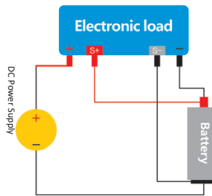
▲ Charge Wiring
